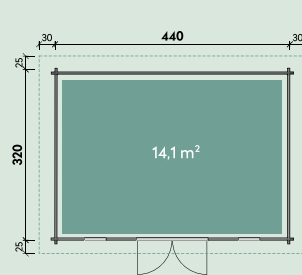
Linda 4432
