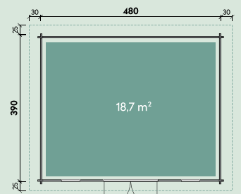
Linda 4839
