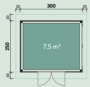
Viola 3025
